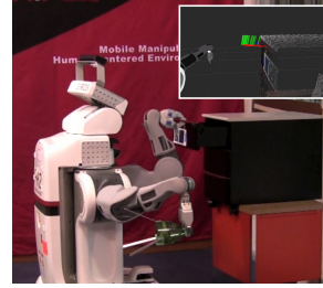
Fig. 1 A robot manipulator autonomously opens a drawer using a kinematic model (visualized in the inset) acquired using the proposed method.
