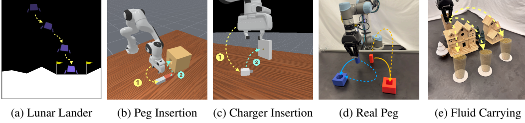
Figure 6: Environment Setting
